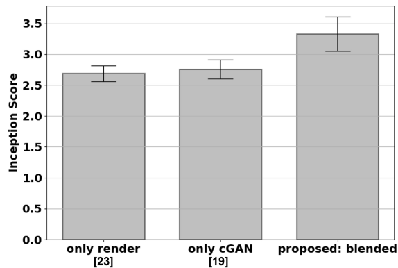
Fig. 7. Inception score [54]. A high Inception score indicates better image quality and higher diversity.
