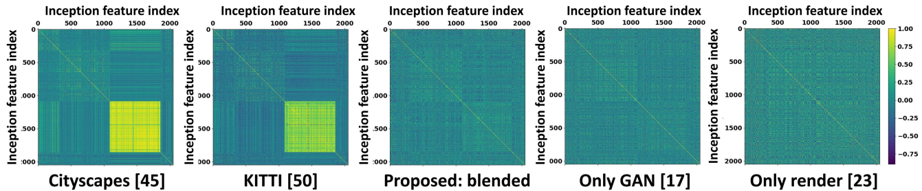
Fig. 6. InceptionV3 feature vector correlation matrices of real and synthetic data. The synthetic dataset that was generated with the proposed blending approach shows a similar correlation pattern with real data. This pattern does not emerge with the only render or only GAN methods.
