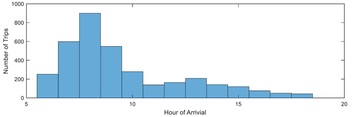
Fig. 2. Histogram of Driver Arrival Times
