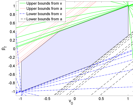
Fig. 5: The upper and lower bounds on p_f due to the acceleration and velocity constraints. Shown as a function of v_0 for t = 0, 0.1, \dots, T_f = 1 . The shaded region shows the feasible values of p_f as a function of v_0 .
