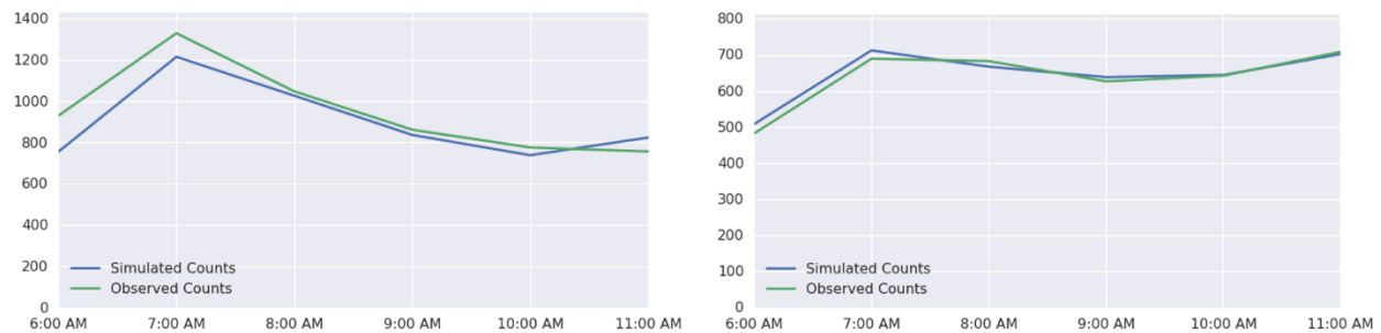
Figure 7 Traffic count calibration on US30 in AM peak.
